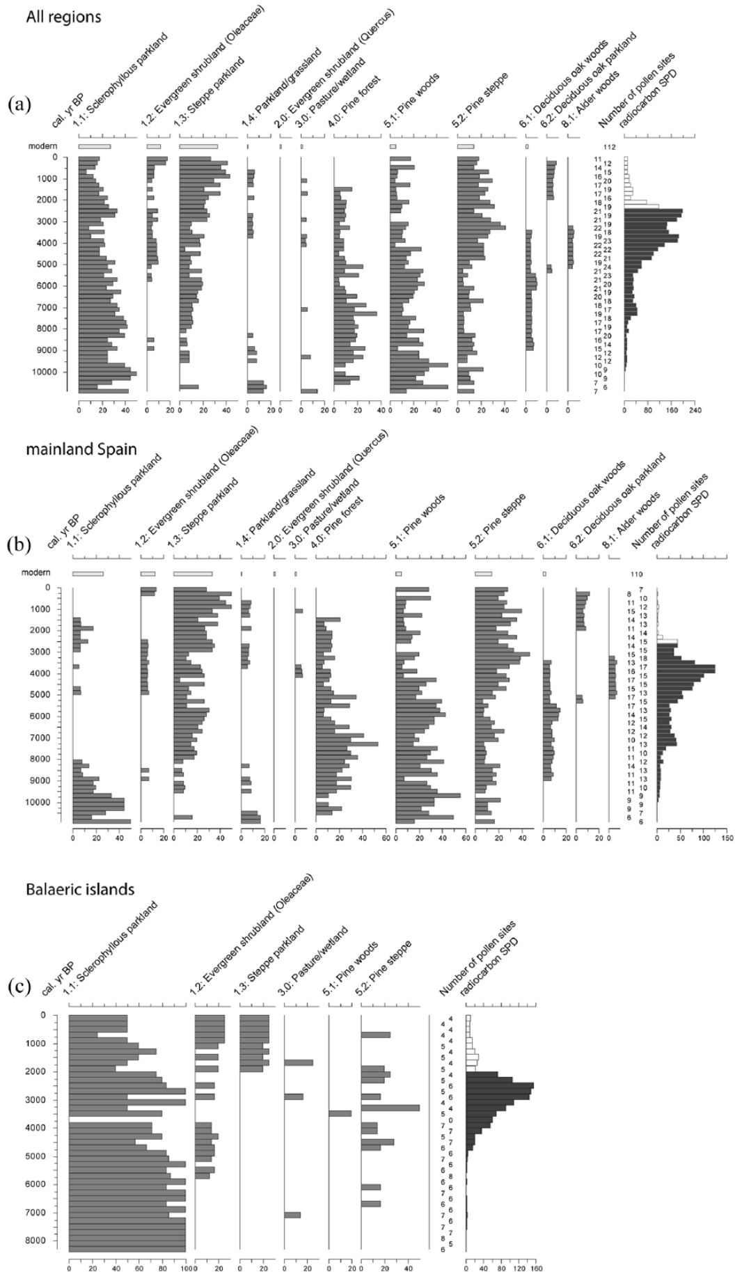
Figure 3. Relative proportions of pollen samples within each vegetation cluster in each time window, for (a) all sites, (b) sites on mainland Spain (north-east and south-east regions combined) and (c) Balearic Islands. Radiocarbon summed probability distributions (SDPs) show results for all dates collated. Time windows with insufficient radiocarbon dates for reliable SDPs are shown in white.
