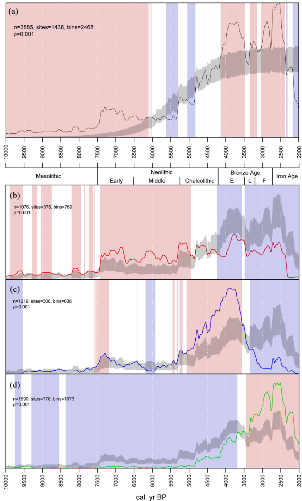
Figure 2. Summed probability distributions (SPDs) of un-normalised calibrated radiocarbon dates (cal. yr BP). (a) all radiocarbon dates against a fitted logistic model (95% confidence); (b) north-east Spain, with SPD for all eastern Spain dates; (c) south-east Spain, with SPD for all Spain dates; (d) Balearic Islands, with SPD for all Spain dates. Vertical bands indicate negative or positive deviations from the null model (a) or all Spain dates (b–d).
