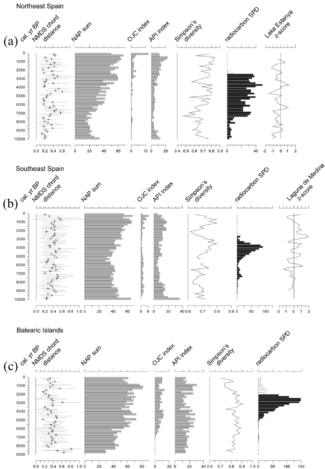
Figure 6. Regional plots of pollen assemblage change (mean NADMS chord distance), sum of non-arboreal pollen types, key anthropogenic indicator groups (API and OJC), Simpson's diversity index, radiocarbon summed probability distributions for each region (a: northeast Spain; b: southeast Spain; c: Balearic Islands) and z-scores for regional proxy-climate records (Lake Estanya: Morellón et al., 2009; Laguna de Medina: Reed et al., 2001).
