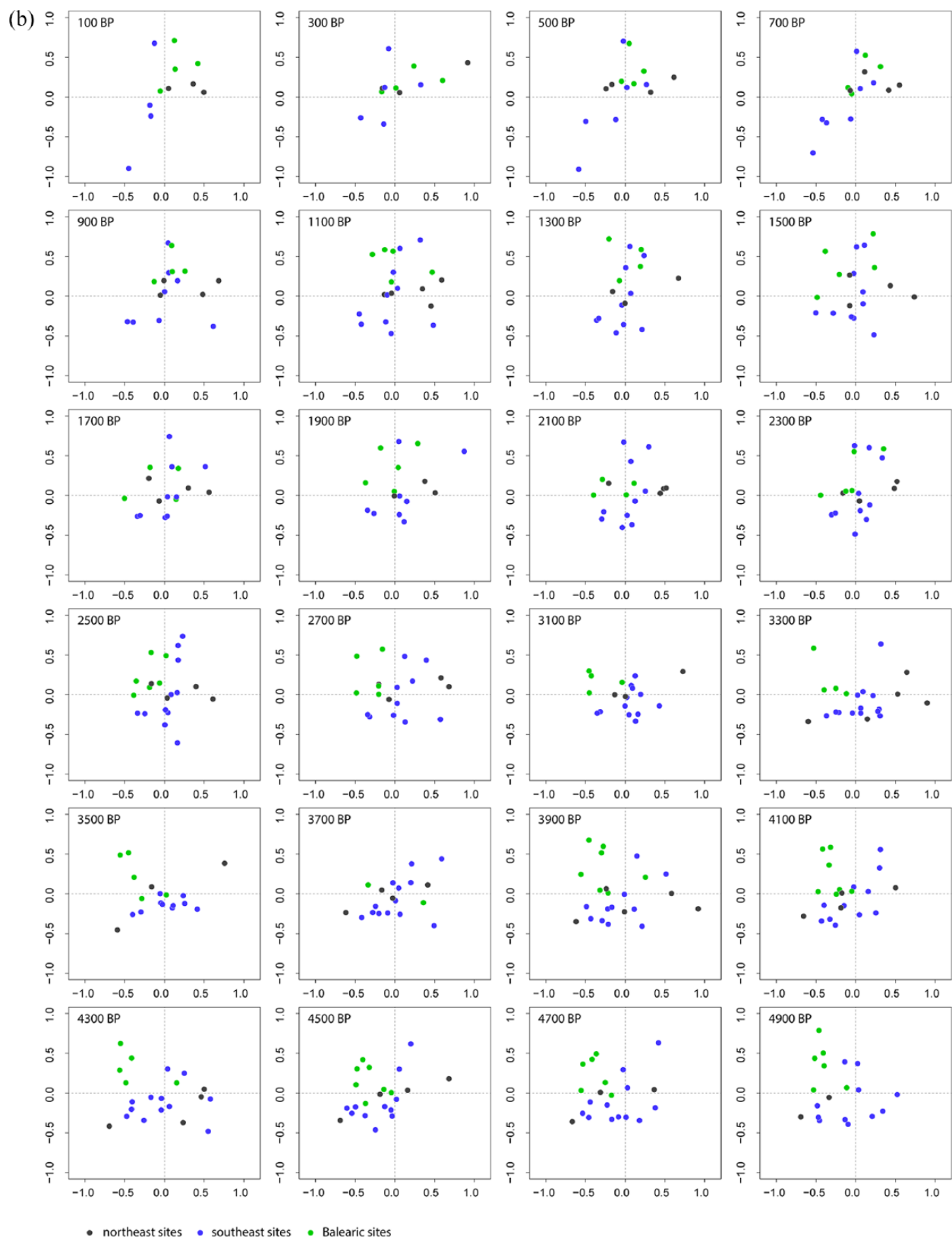
Figure 5. Site plots from non-metric multidimensional scaling (NMDS) analysis in each time interval. (a) 9900–5100 cal. yr BP and (b) 4900–100 cal. yr BP. Plot shows axis 1 versus 2 scores. Green is Balearic sites, black north-east Spanish sites and blue south-east Spanish sites. (labelled version in Supplementary Information, available online).
