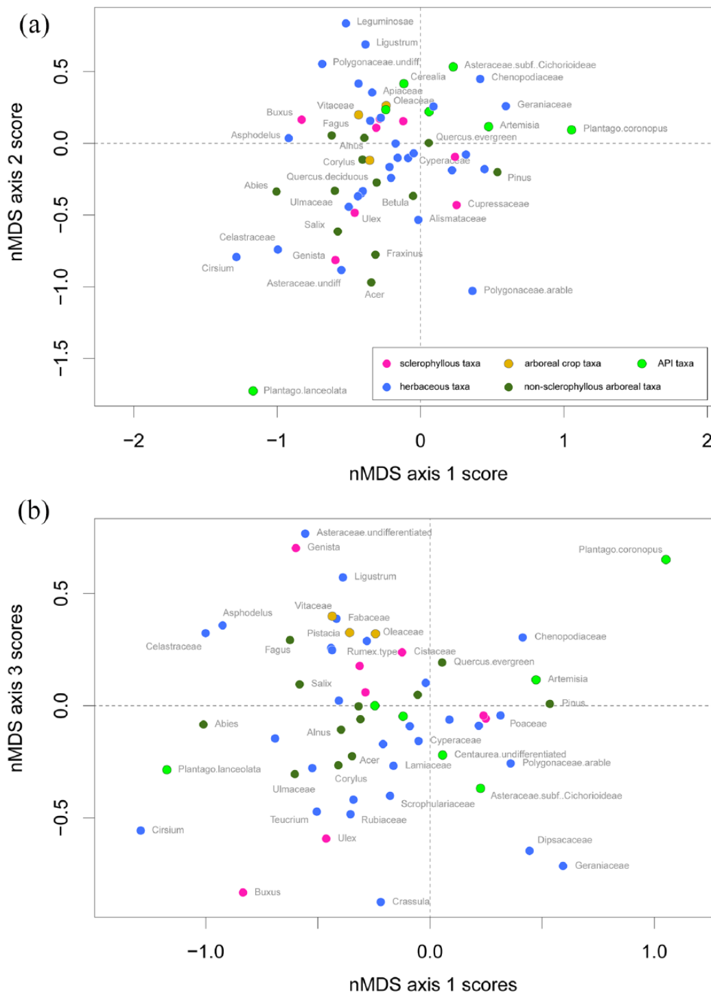
Figure 4. Taxa plots from non-metric multidimensional scaling (NMDS) analysis of all sites, showing (a) axis 1 versus 2 and (b) axis 1 versus 3. Taxa are grouped into broad ecological or anthropogenic indicator classes.
