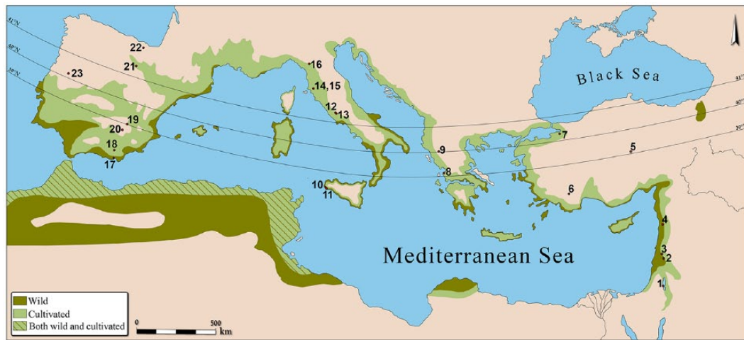
Figure 1. Geographical distribution of wild olive ( Olea europaea subsp. oleaster ) and cultivated olive in the Mediterranean Basin (redrawn from Carrión et al. (2010) and Lavee and Zohary (2011)). Numbers represent the sites used in the palynological diagrams (Figures 3–5): (1) Dead Sea, (2) Sea of Galilee, (3) Lake Hula, (4) Al Jourd, (5) Eski Acigöl, (6) Gölhisar Gölü, (7) Lake Iznik, (8) Lake Voukaria, (9) Lake Gramousti, (10) Lago Preola, (11) Gorgo Basso, (12) Albano, (13) Nemi, (14) Accesa (center), (15) Accesa (edge), (16) Lago Padule, (17) San Rafael, (18) Baza, (19) Villaverde, (20) Siles, (21) Laguna Negra, (22) Saldropo, and (23) Charco da Candieira. The pollen data primarily derive from collaborators (Table 1) as well as the European Pollen Database (EPD, Leydet, 2007–2017).
