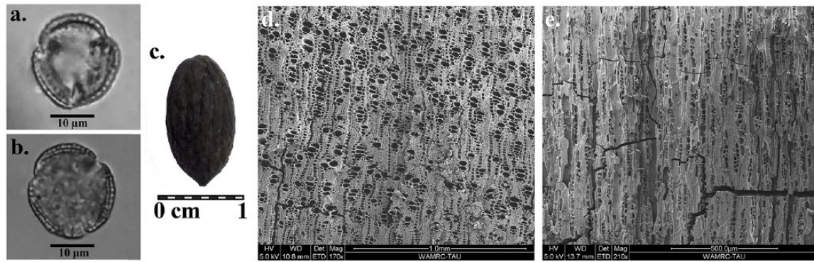
Figure 2. Macro- and micro-botanical evidence of olive: (a) a fossil pollen grain of wild Olea extracted from a stratum dated to the end of the Last Glacial period at the Epipaleolithic site of Jordan River Dureijat (southern Levant). (b) A fossil pollen grain of cultivated Olea recovered from the royal garden in Herod the Great's tomb complex at the semi-desert site of Herodium (southern Levant). Olea europaea pollen grains are usually sub-transverse to spheroidal, have three short colpi, relatively thick exine and nexine, and reticulate ornamentation varying from fine to coarse. (c) An olive endocarp collected from a well at Kfar Samir (southern Levant), dated to the late Pottery Neolithic (~7600–7000 yBP; Galili et al., 2018); so far, Kfar Samir provides the earliest direct evidence in the world for olive oil production (Galili et al., 1997). (d) and (e) are SEM images showing two axes, transverse (d) and tangential (e), of olive wood charcoal collected from the Chalcolithic site of Tel Tsaf (southern Levant, early 7th millennium BP), where evidence for early fruit tree cultivation has been found (olive, fig and grapes; Langgut and Benzaquen, in press). The charcoal exhibits the typical features of the olive's woody anatomy: in the transverse (d), note the diffuse porous, round to angular vessels (generally between 30 and 60 \mu\text{m} in diameter) frequently arranged in radial multiples of up to six or in clusters; and in the tangential (e), note the 1–3 seriate rays with uniseriate portions as large as multiseriate portions and vessel member lengths less than 350 \mu\text{m} . Pollen images are part of the collection of the Steinhardt Museum of Natural History, Tel Aviv University.
