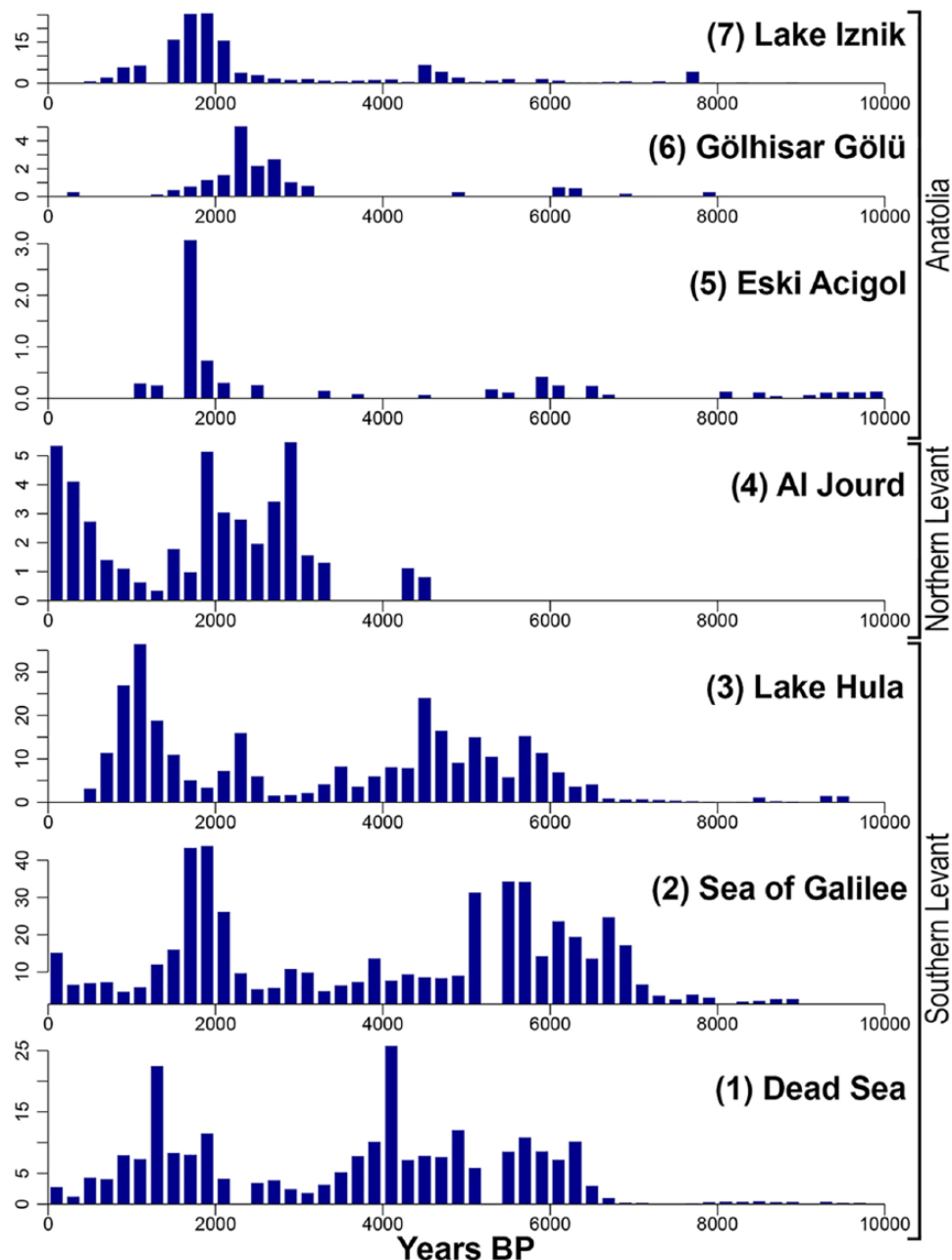
Figure 3. Olea pollen percentages during the Holocene in the Eastern Mediterranean Levant. Note the different percentage of vertical scales.
