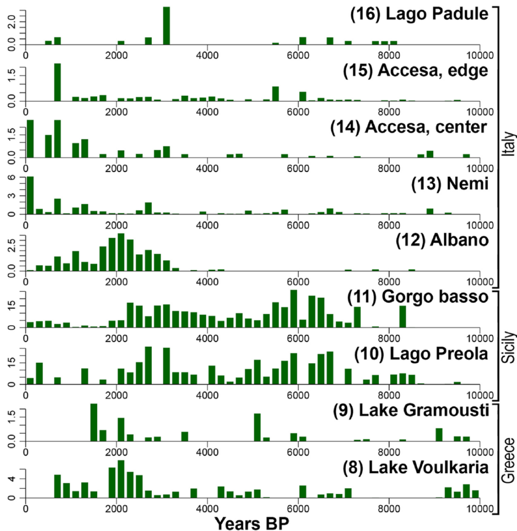
Figure 4. Olea pollen percentages during the Holocene in the Central Mediterranean. Note the different percentage of vertical scales.
