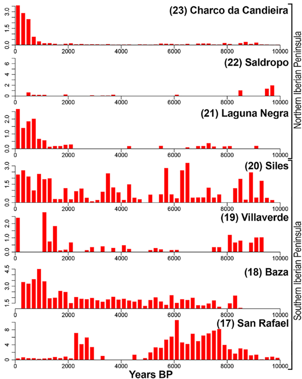
Figure 5. Olea pollen percentages during the Holocene in the Western Mediterranean. Note the different percentage of vertical scales.
