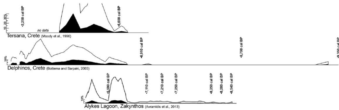
Figure 7. Palynological records from the islands of Crete and Zakynthos demonstrating a significant increase in olive pollen at ~6000 yBP. We believe that this rise is indicative of olive horticulture in southern Greece. The sudden dramatic increase was not accompanied by pollen rise of other broadleaved trees and therefore cannot be regarded as climate related. The radiocarbon dates provided with the Tersana and Delphinios records were recalibrated using OxCal v.4.3.2 (Bronk Ramsey, 2017). Olea pollen curves were drawn based on Moody et al. (1996) – the Tersana record, Bottema and Sarpaki (2003) – the Delphinios record and Avramidis et al. (2013) – the Alykes Lagoon record. The solid black line is a fivefold exaggeration curve used to show low Olea percentages.
