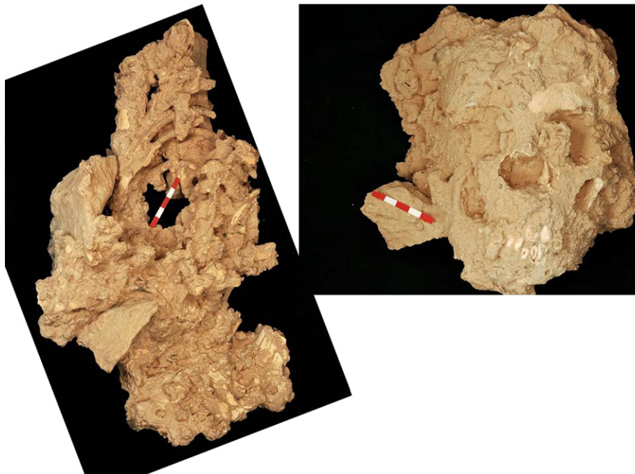
Fig. 12. SP-97 skeleton and skull partly cleaned.
