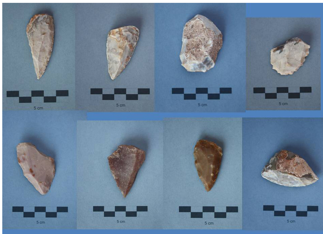
Fig. 8. Mousterian artifacts, mostly from upper finer sedimentary deposit (A in Fig. 7). Scrapers and points were made on flint of good quality. No flint outcrops are known on Cabezo Gordo and the artifacts were doubtless brought to the site, together with small amounts of the raw material for knapping although cores and knapping debris are infrequent.
