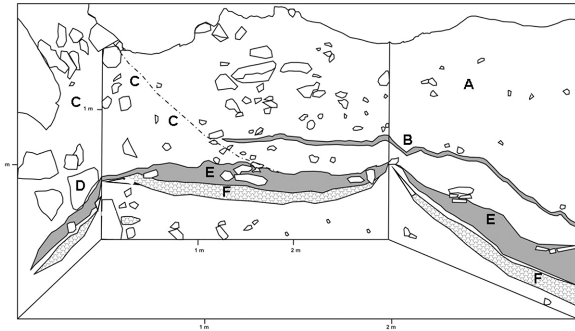
Fig. 7. Stratigraphy of the upper cutting. A = upper finer sedimentary deposit. B = upper grey layer. C = cemented scree and rock tumble of conglomerate A; the broken line indicates the slope and although it hardly impinged at all on the northern section at the rear of the figure, its presence was well demonstrated in standing sections in the foreground before they were removed at excavation. D = block of conglomerate A containing part of SP-97 (see Fig. 11). E = lower grey layer. F = conglomerate B.
