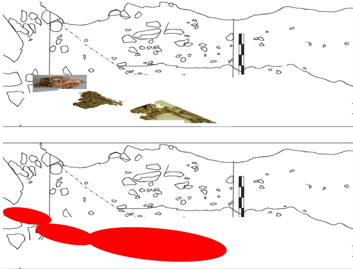
Fig. 9. Situation of the SP-96 skeleton. From left to right the three red ovals indicate approximately where the skull, thoracic skeleton and lower limbs lay, in an inclined position. (For interpretation of the references to colour in this figure legend, the reader is referred to the web version of this article.)
