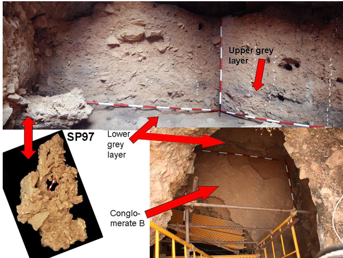
Fig. 11. Left: block of conglomerate A containing a part of the SP-97 skeleton which is shown below partly cleaned. Lower right: conglomerate B during excavation.
