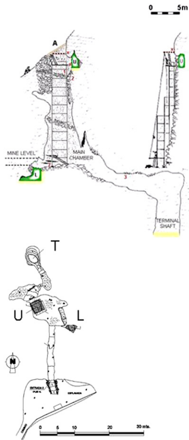
Fig. 3. Main shaft, sketch of vertical elevation, scale plan. A = mouth of main shaft. U = upper cutting. L = lower cutting. T = terminal shaft. The plan includes the artificial terrace on the hill-side, in front of the entrance to the mine tunnel, formed by rubble and soil we have excavated and sieved.
